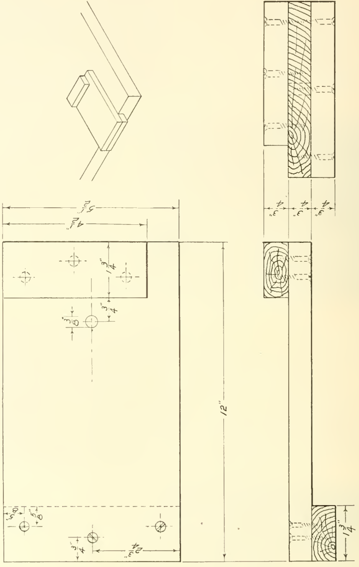
Bench Hook
